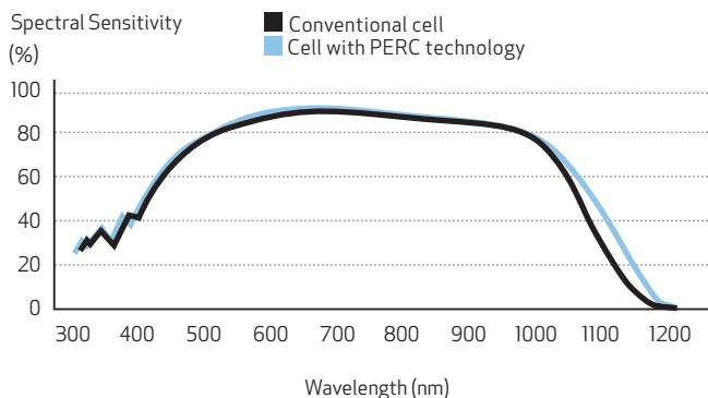
Fig. 5: PERC technology increases cell sensitivity to wavelengths between 1000 & 1180 nm.
